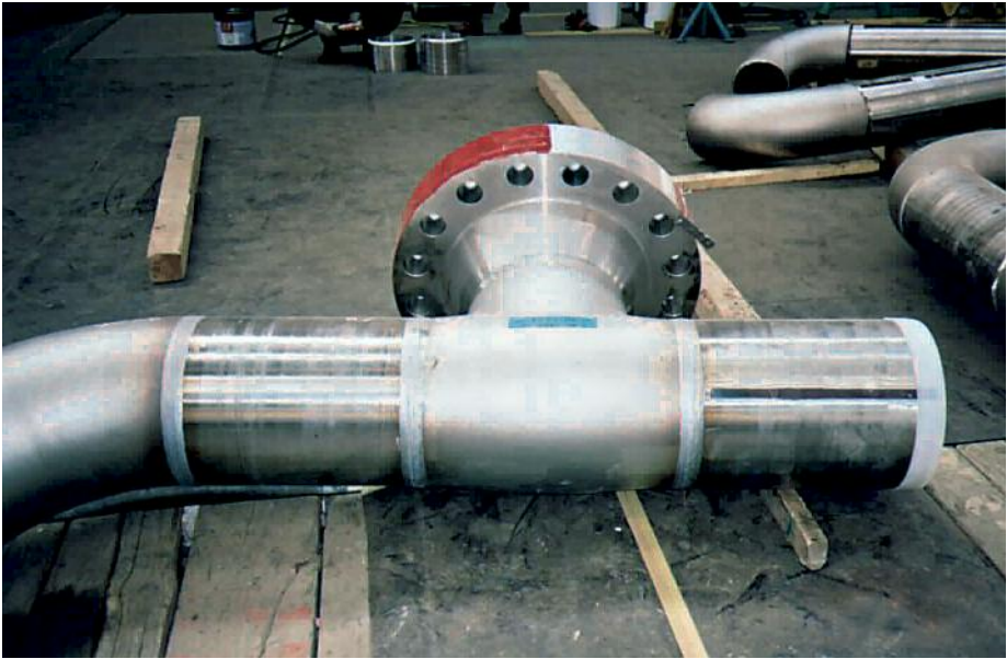
2205双相不锈钢T形法兰 © Arco Exploration and Production Technology
